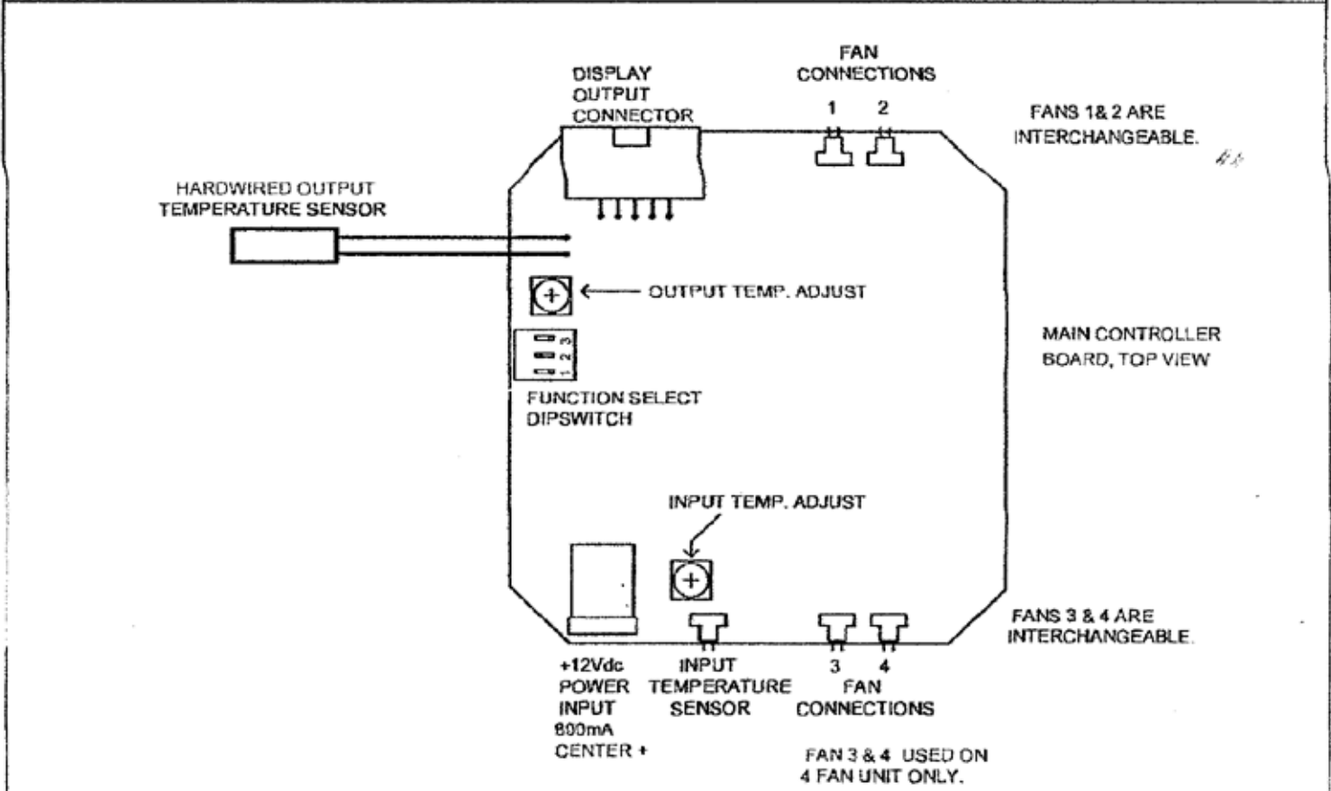
MAIN ISOBOX CONTROL BOARD CONNECTION DIAGRAM
