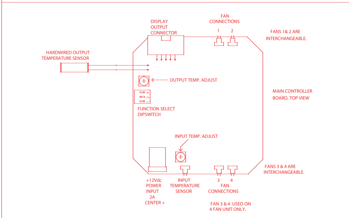
MAIN ISOBOX CONTROL BOARD CONNECTION DIAGRAM
