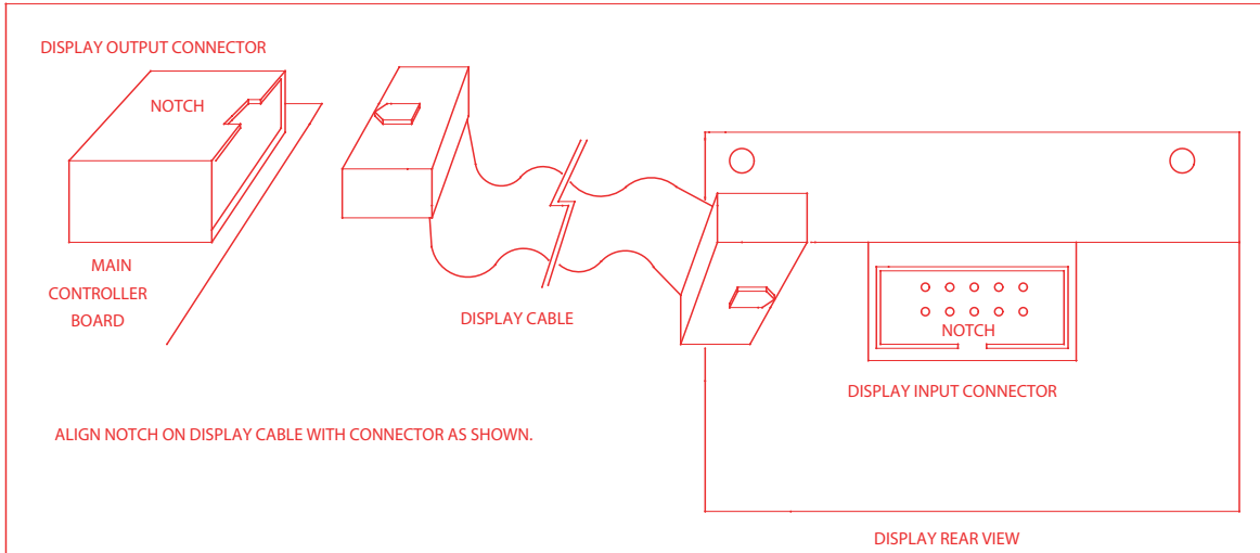
ISOBOX DISPLAY CONNECTION DIAGRAM
